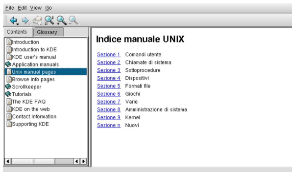
Figura 28.132. Khelpcenter.
